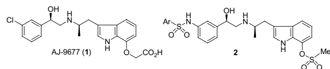
Figure 1. Structures of tryptamine-based human \beta_3 -AR agonists.
