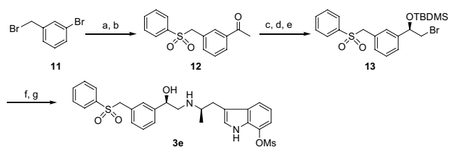
Scheme 3. Reagents: (a) benzenesulfonic acid sodium salt, DMF; (b) butyl vinyl ether, K_2CO_3 , Pd(OAc)_2 , 1,3-bis(diphenylphosphino)propane, DMF, H_2O ; (c) phenyltrimethylammonium tribromide, THF; (d) ( R )-2-methyl-CBS-oxazaborolidine, BH_3 , THF; (e) TBDMSCl, imidazole, DMF; (f) 7 , i - Pr_2NEt , KI, MeCN; (g) 4 N HCl–AcOEt, EtOH.
