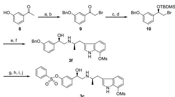
Scheme 2. Reagents: (a) benzyl bromide, K 2 CO 3 , DMF; (b) phenyltrimethylammonium tribromide, THF; (c) ( R )-2-methyl-CBS-oxazaborolidine, BH 3 , THF; (d) TBDMSCl, imidazole, DMF; (e) 7 , i -Pr 2 NEt, KI, MeCN; (f) 4 N HCl–AcOEt, EtOH; (g) (Boc) 2 O, CHCl 3 ; (h) H 2 , 20% Pd(OH) 2 , EtOH; (i) benzenesulfonyl chloride, Et 3 N, CH 2 Cl 2 ; (j) 4 N HCl–AcOEt.
