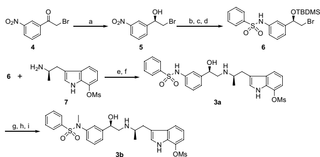
Scheme 1. Reagents: (a) ( R )-2-methyl-CBS-oxazaborolidine, BH 3 , THF; (b) TBDMSCl, imidazole, DMF; (c) Fe, NH 4 Cl, EtOH, H 2 O; (d) benzenesulfonyl chloride, pyridine, CH 2 Cl 2 ; (e) i -Pr 2 NEt, KI, MeCN; (f) 4 N HCl–AcOEt, EtOH; (g) (Boc) 2 O, CHCl 3 ; (h) MeI, K 2 CO 3 , DMF; (i) 4 N HCl–AcOEt.
